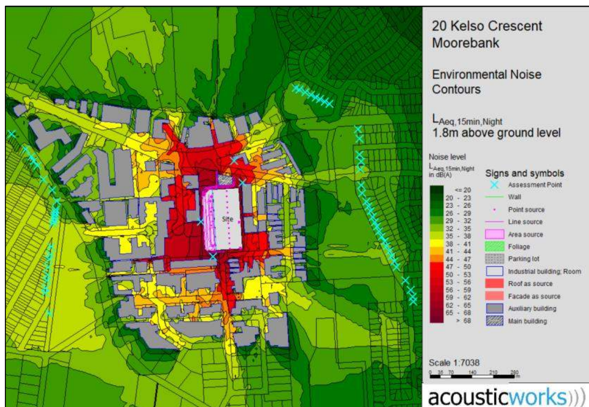
Figure 36. Environmental Noise Contours - LAeq 15 min Night - 1.8m above ground level (Source: Acoustic Works, 2024)
