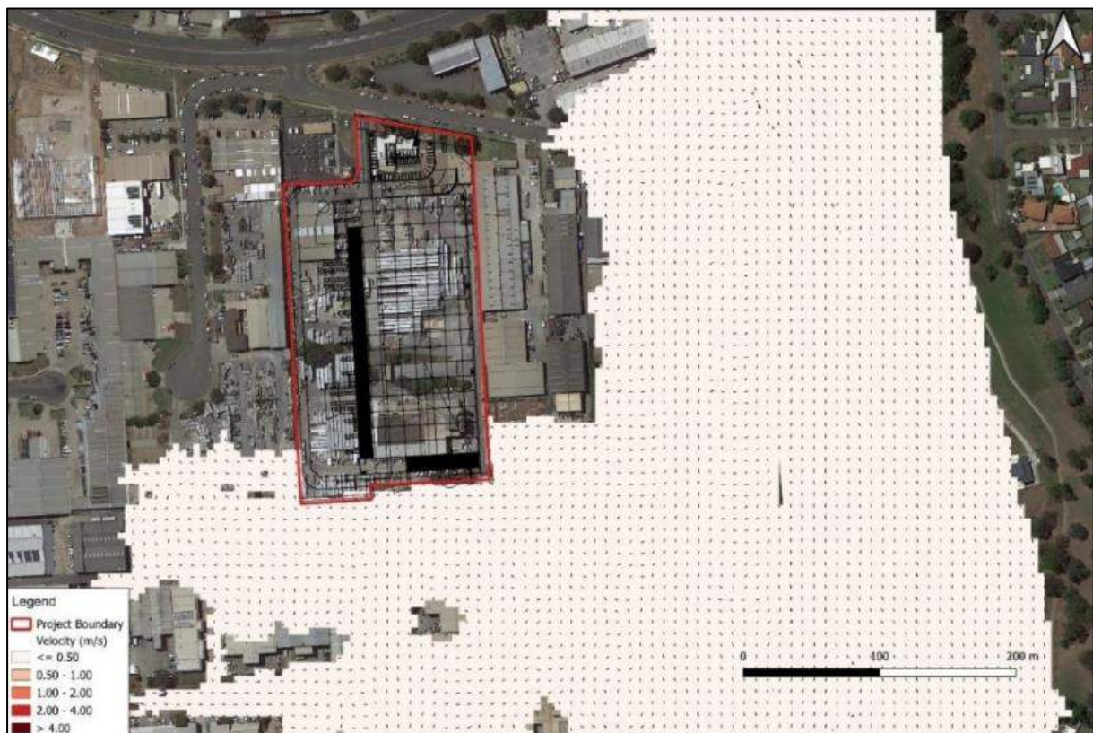
Figure 43. Post Development 1% AEP Flood Velocities (Source: TTW, 2023)
