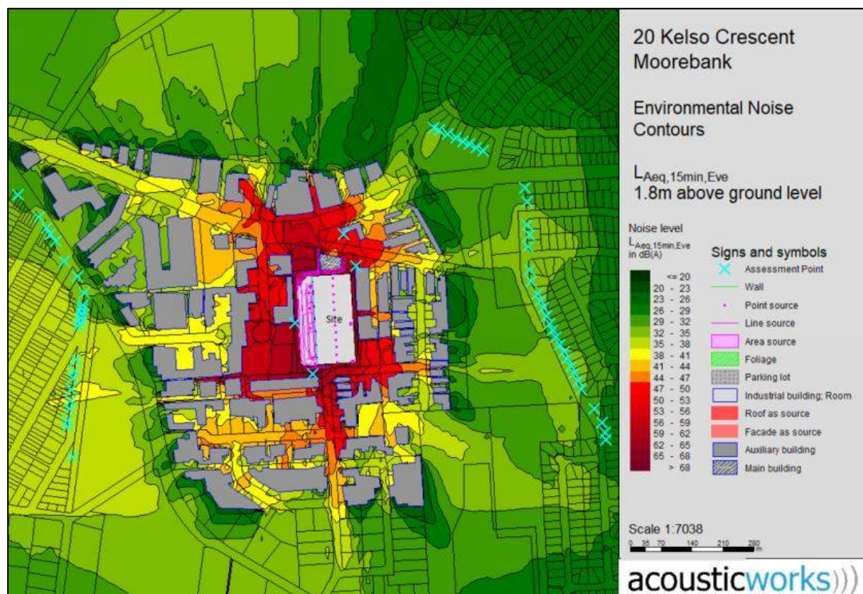
Figure 35. Environmental Noise Contours - LAeq 15 min Evening - 1.8m above ground level (Source: Acoustic Works, 2024)
