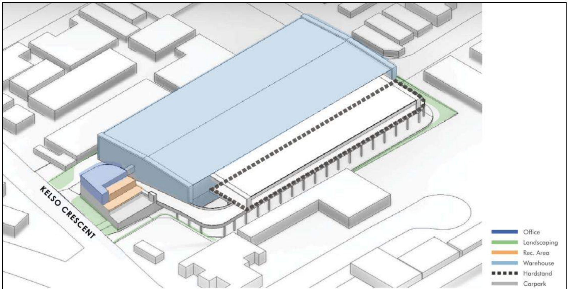
Figure 20. Proposed Building Configuration Drawing (Source: Nettletontribe, 2023)
