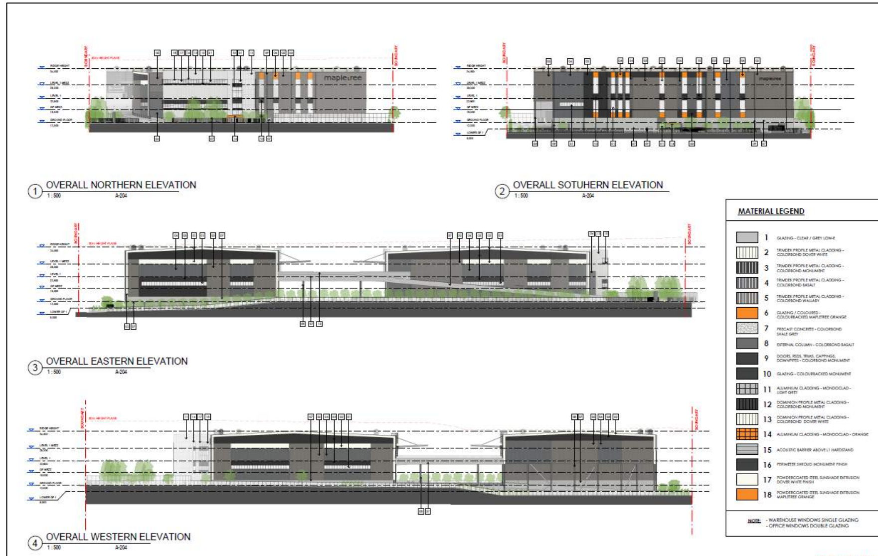
Figure 10: Elevations (Source: PACE Architects, 2025)
