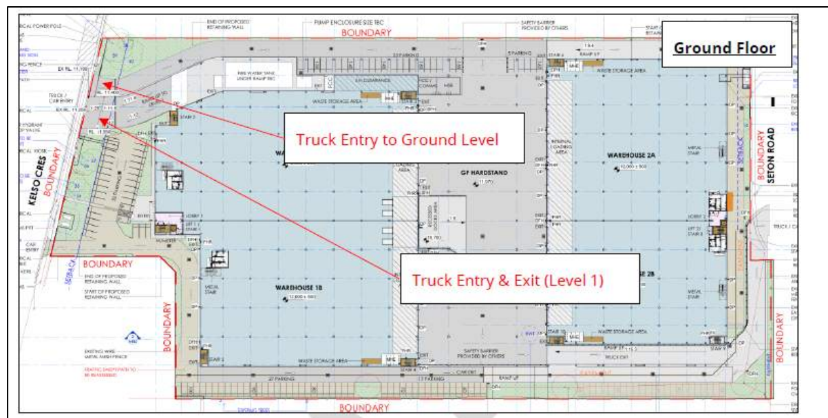
Figure 14: Truck Access and Egress - Ground Floor (Source: PACE Architects, 2025)
