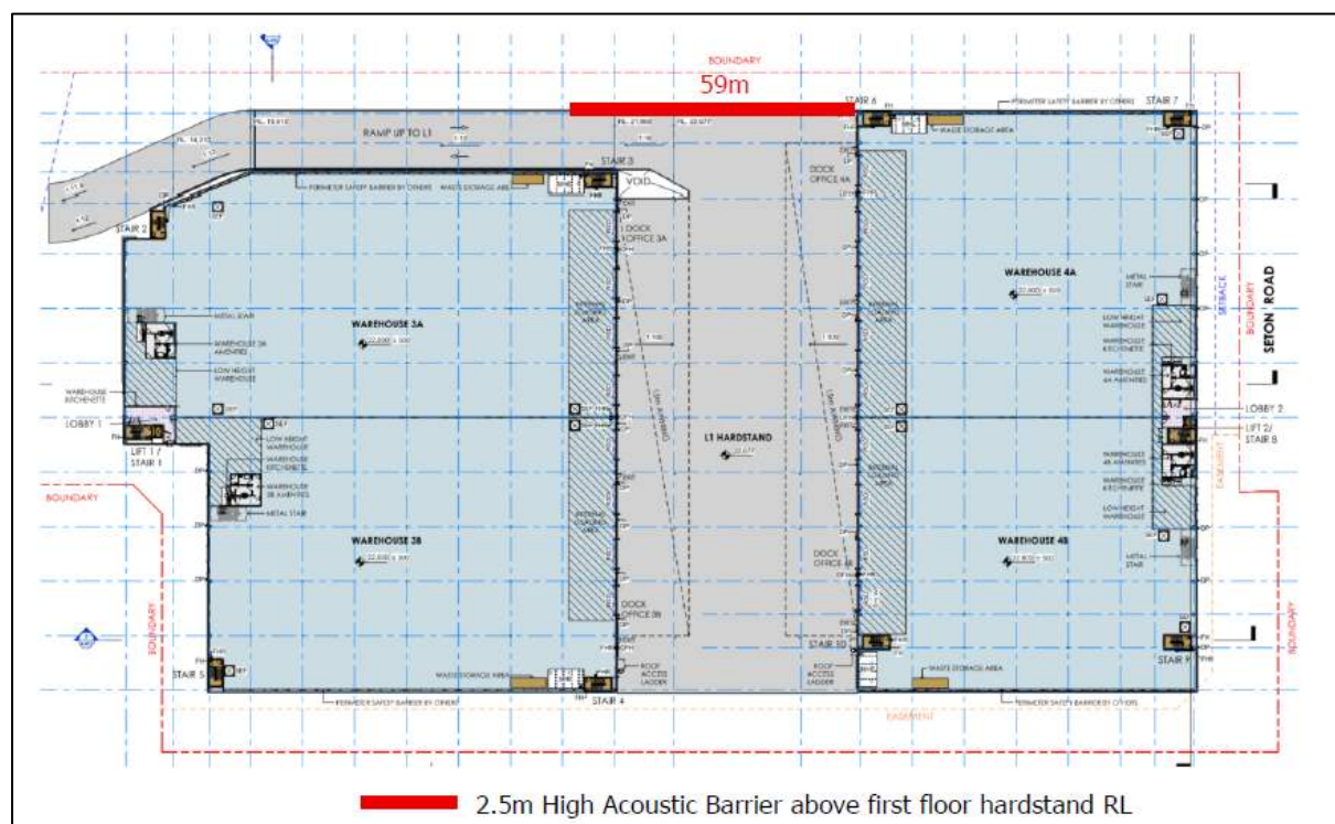
Figure 18: Recommended Acoustic Barriers (Source: Acoustic Works, 2025)
