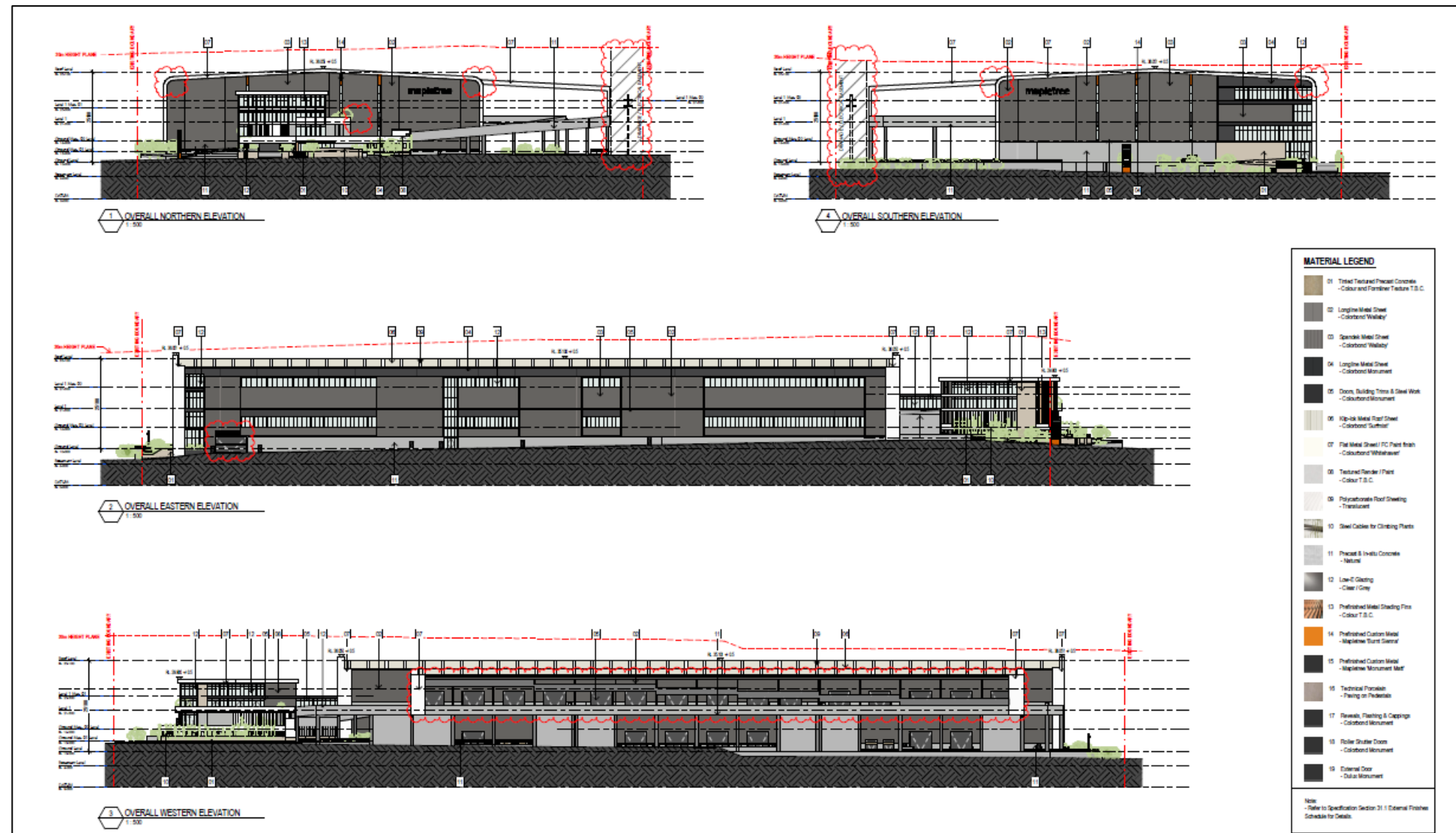
Figure 9: Elevations (Source: Nettleton Tribe, 2024)
