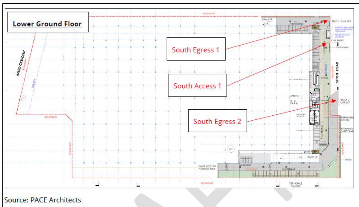
Figure 13: Car Park Access and Egress – Lower Ground Floor (Source: PACE Architects, 2025)
