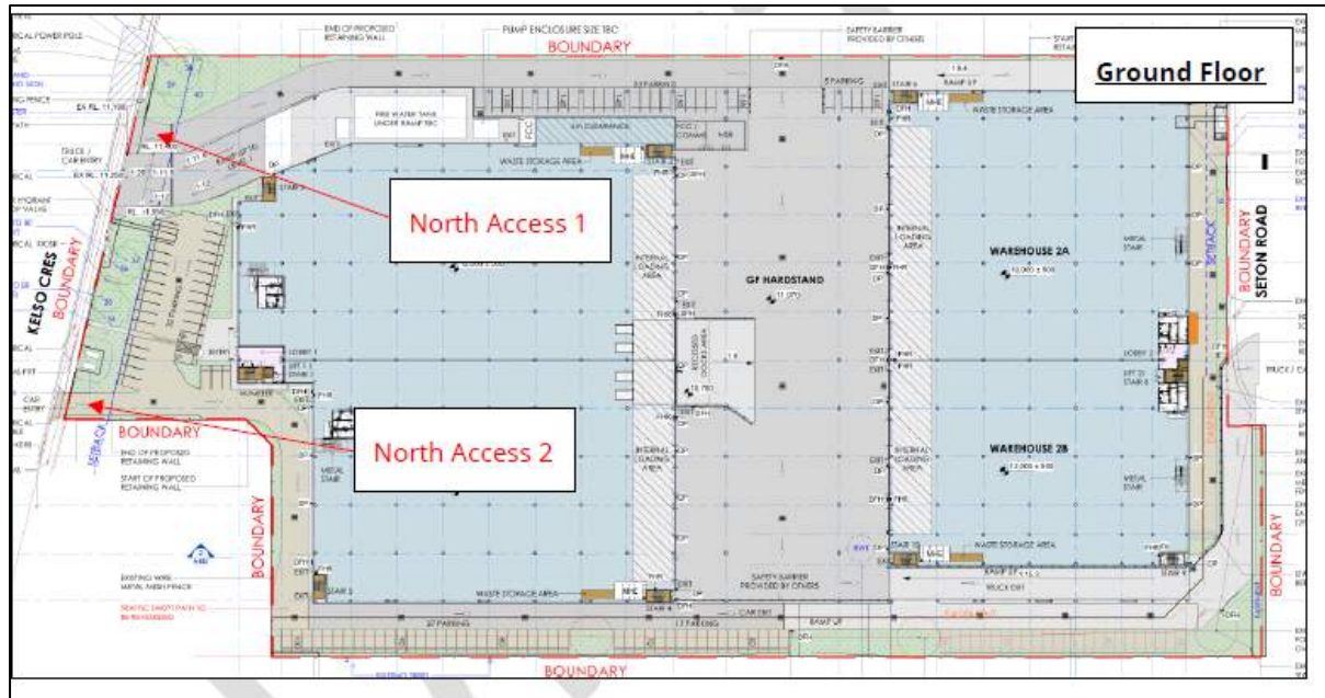
Figure 12: Car Park Access and Egress – Ground Floor (Source: PACE Architects, 2025)
